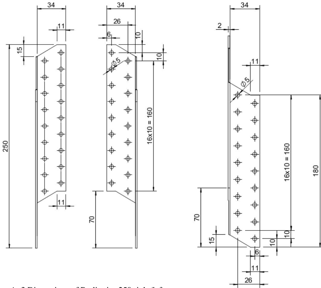
Figure A. 3 Dimensions of Purlin ties 250 right/left
