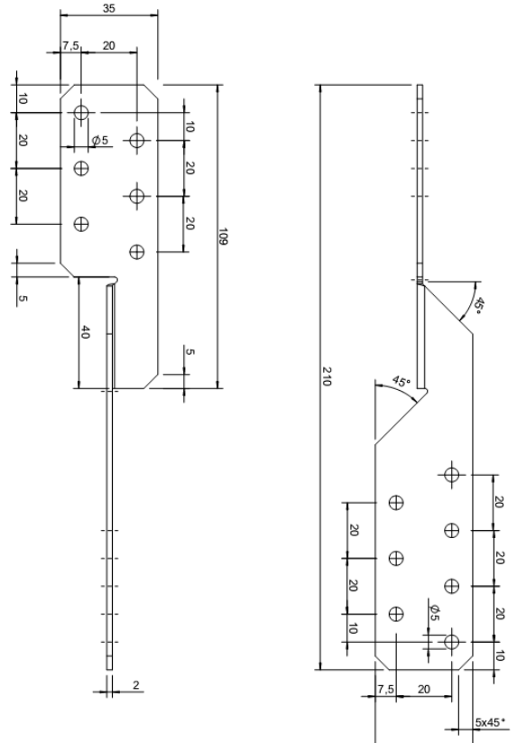
Figure A.8 Dimensions of Purlin ties 210 universal
