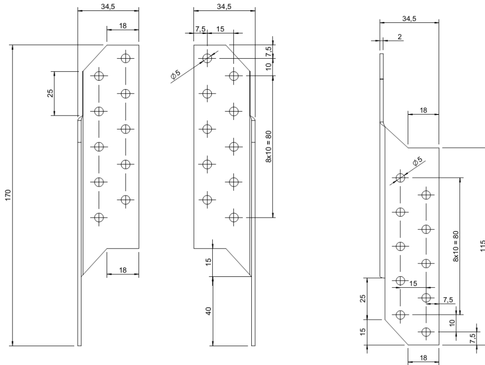
Figure A. 1 Dimensions of Purlin ties 170 right/left
