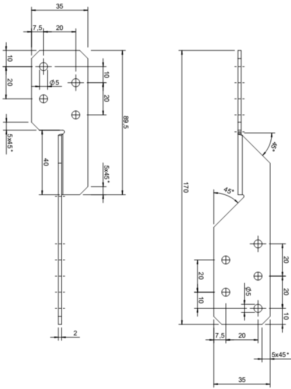
Figure A.7 Dimensions of Purlin ties 170 universal
