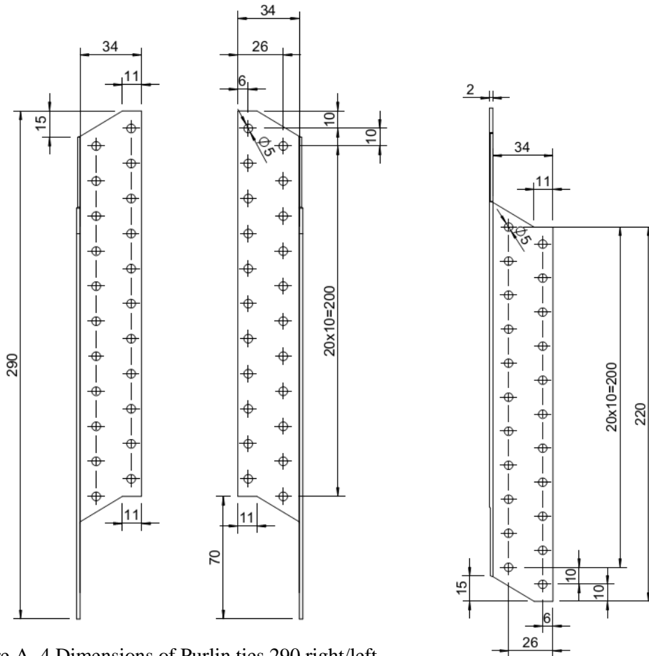
Figure A. 4 Dimensions of Purlin ties 290 right/left
