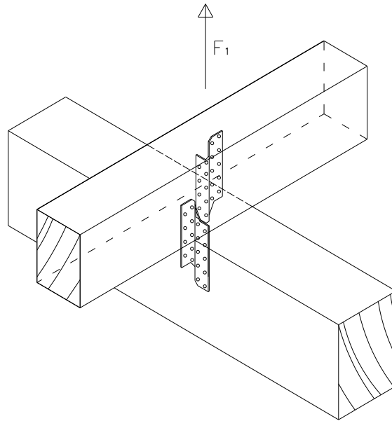
Figure A. 13 Typical installation
