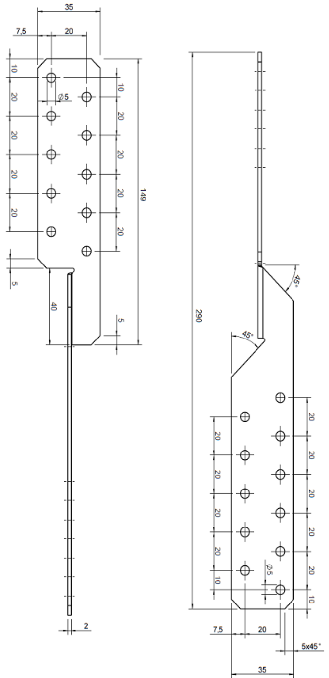
Figure A.10 Dimensions of Purlin ties 290 universal
