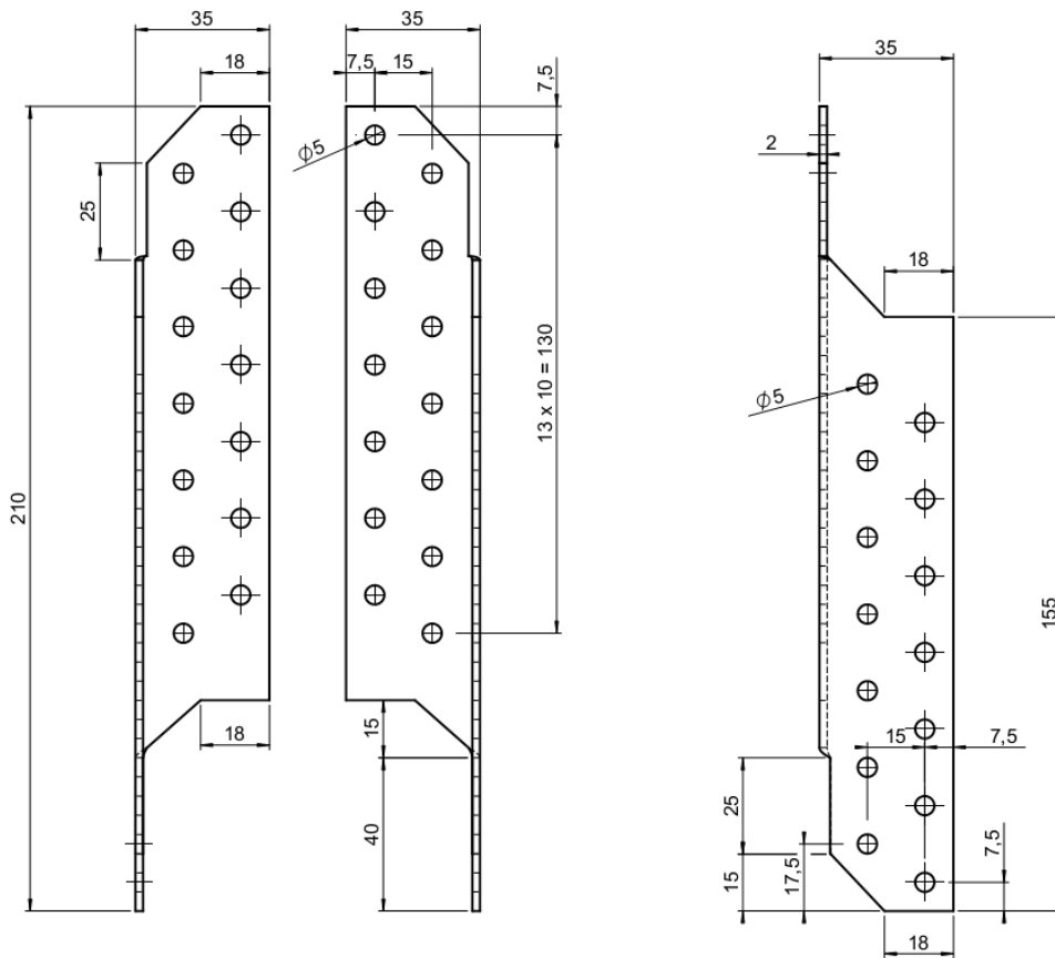
Figure A. 2 Dimensions of Purlin ties 210 right/left
